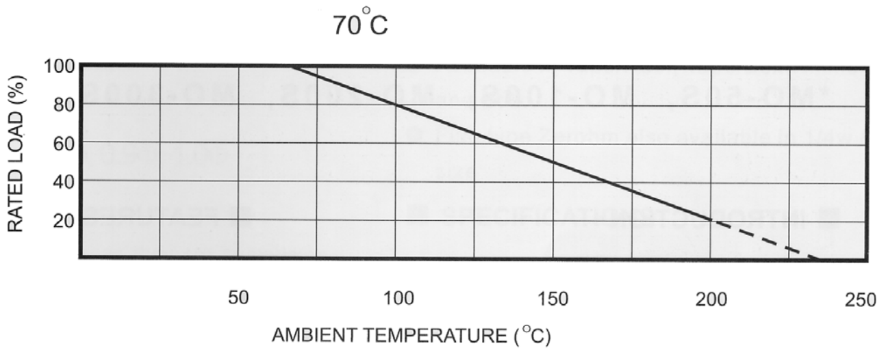
FIG.1 Derating Curve
